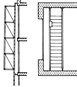
2 Parallel travel safety ladders (for 3 or 4 storeys)
